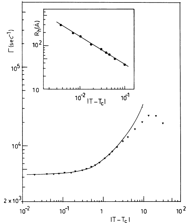
FIG. 3. Log-log plot of the relaxation rate of the critical concentration ( \theta = 90^\circ ) vs T_C - T ; the dots are the experimental results, whereas the solid line is the calculation in terms of the prediction of mode coupling including background effects. In the inset is reported the power-law divergence of the hydrodynamic radius R_h . Temperature is measured in degrees Kelvin.
